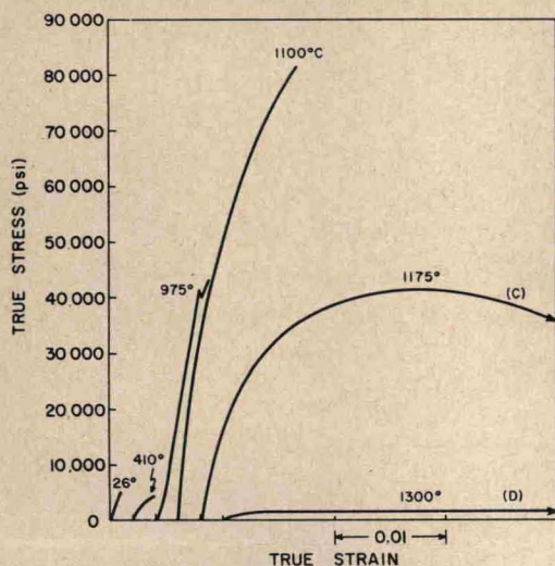
Fig. 1. Typical stress-strain curves of talc in compression at different temperatures.
